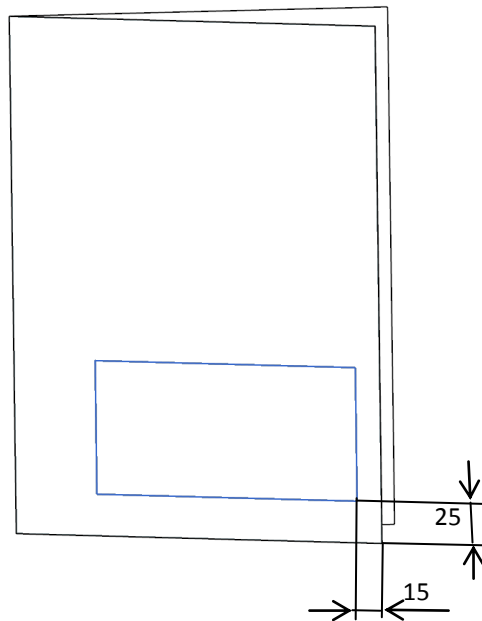
Fig 1. Method of allocating the title block on the folder cover.
